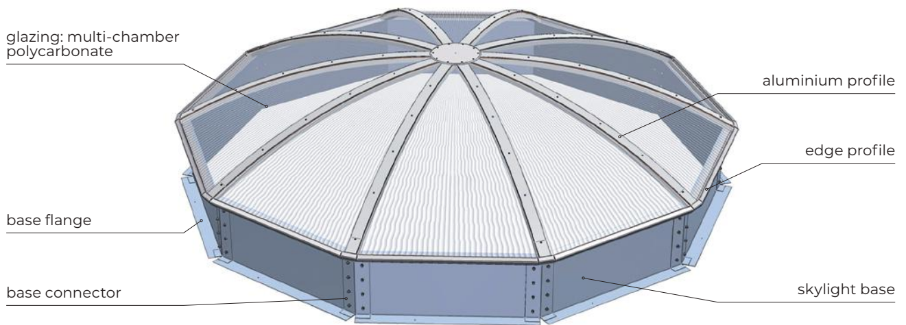
Fig. 104 mcr PROLIGHT dome skylight design
