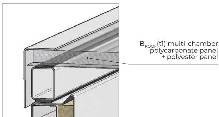
Fig. 55 Vent glazing: multi-chamber polycarbonate panel + polyester panel
