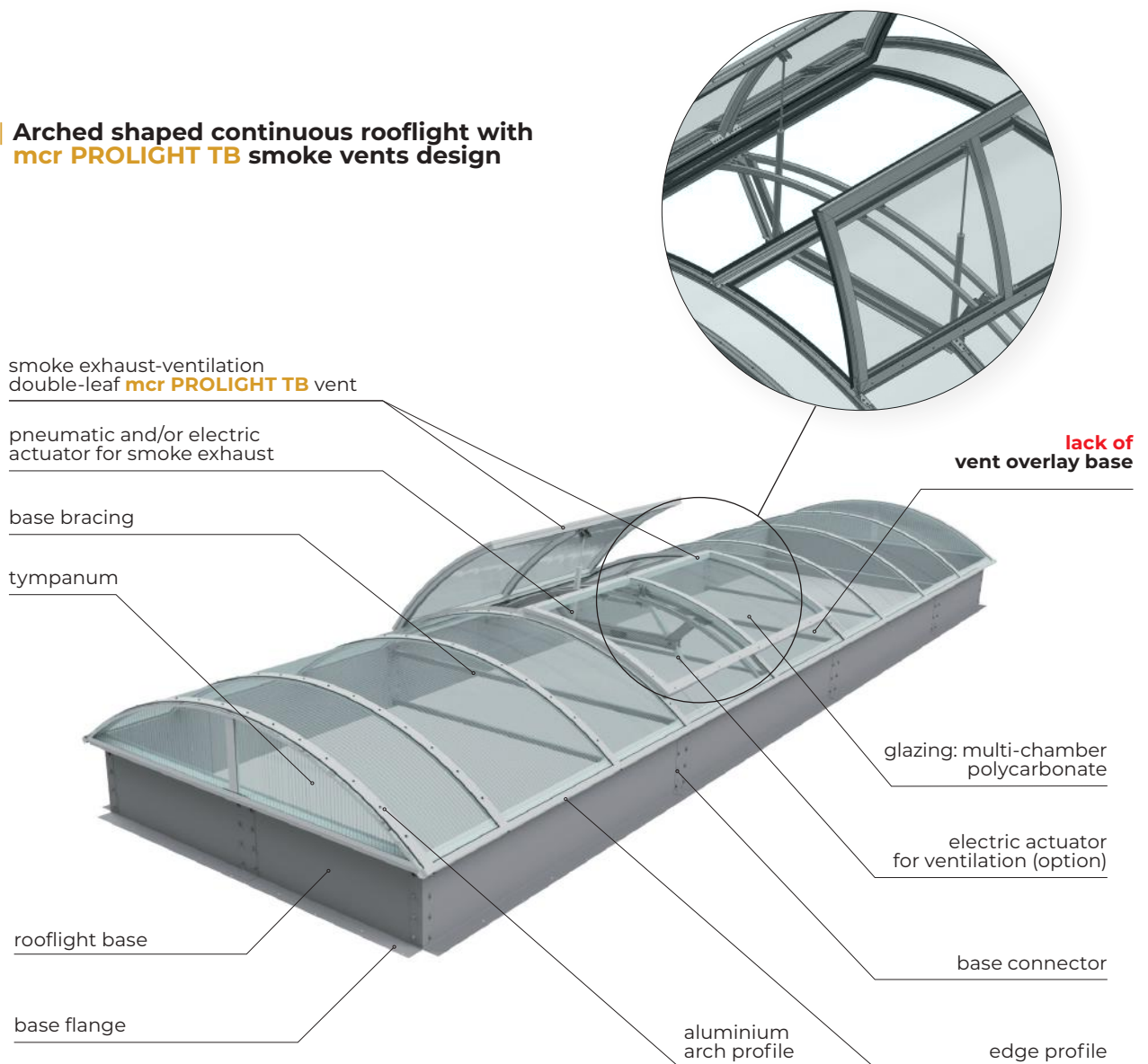
Rys. 88 Design of mcr PROLIGHT arch shaped continuous rooflight with integrated mcr PROLIGHT TB smoke exhaust and daily ventilation double-leaf vent
