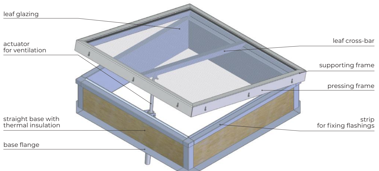
Fig. 28 mcr PROLIGHT C ventilation vent design with electric actuator for ventilation
