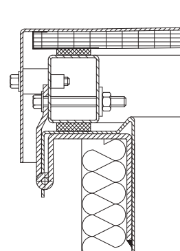
Fig. 50 Vent section, glazing: ALU envelope cover with multi-chamber polycarbonate
