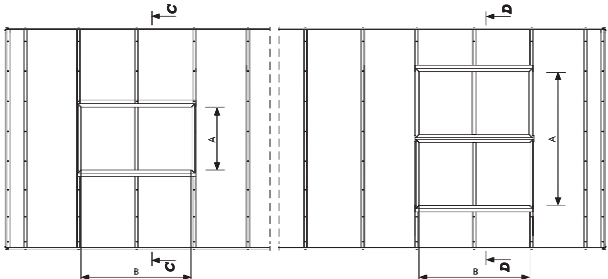
Fig. 87 Top view of mcr PROLIGHT arch shaped continuous rooflight with integrated smoke exhaust and daily ventilation single and double-leaf vent
