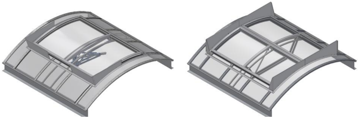
Fig. 139 Wind deflectors in single-leaf and double-leaf smoke vent installed in continuous rooflight
