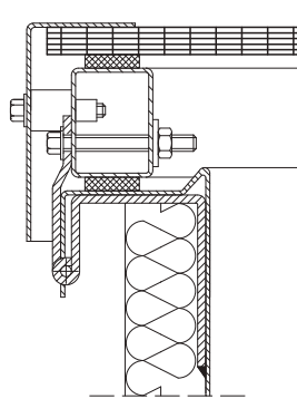
Fig. 36 Vent glazing: multi-chamber polycarbonate panel
