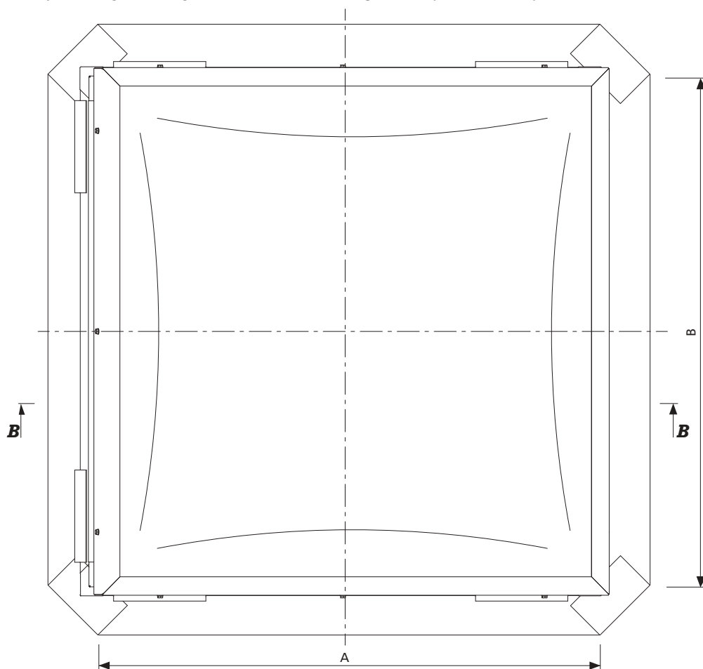
Fig. 33 Top view of mcr PROLIGHT NG-A ventilation vent with skew base in open position, dimensions in mm
