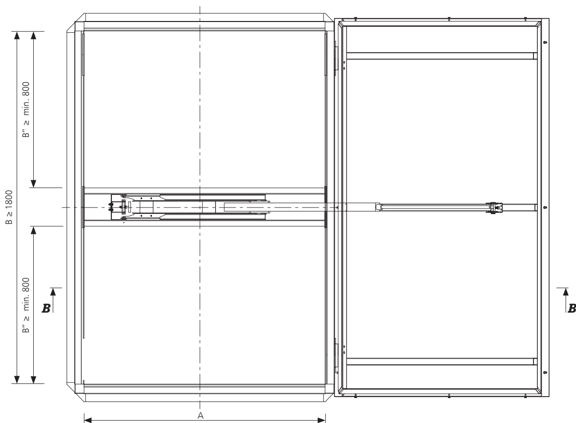
Rys. 62 Top view of the mcr PROLIGHT C or E smoke vent with a roof access option in the open position, dimensions in mm
