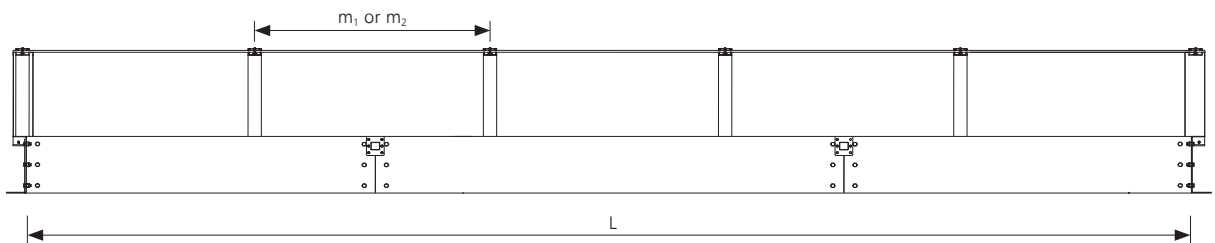
Fig. 82 Cross section B-B of mcr PROLIGHT arch shaped continuous rooflight
