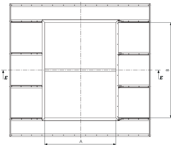
Fig. 91 Top view of arch shaped continuous rooflight with integrated mcr PROLIGHT TB smoke exhaust and daily ventilation single and double-leaf vent
