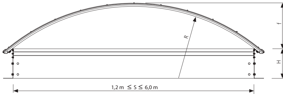
Fig. 81 Cross section A-A of mcr PROLIGHT arch shaped continuous rooflight
