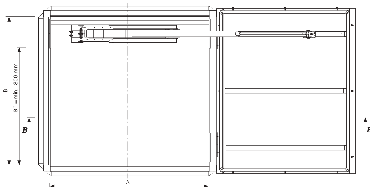
Fig. 59 Top view of mcr PROLIGHT smoke vent with roof access function in open position, dimensions in mm
