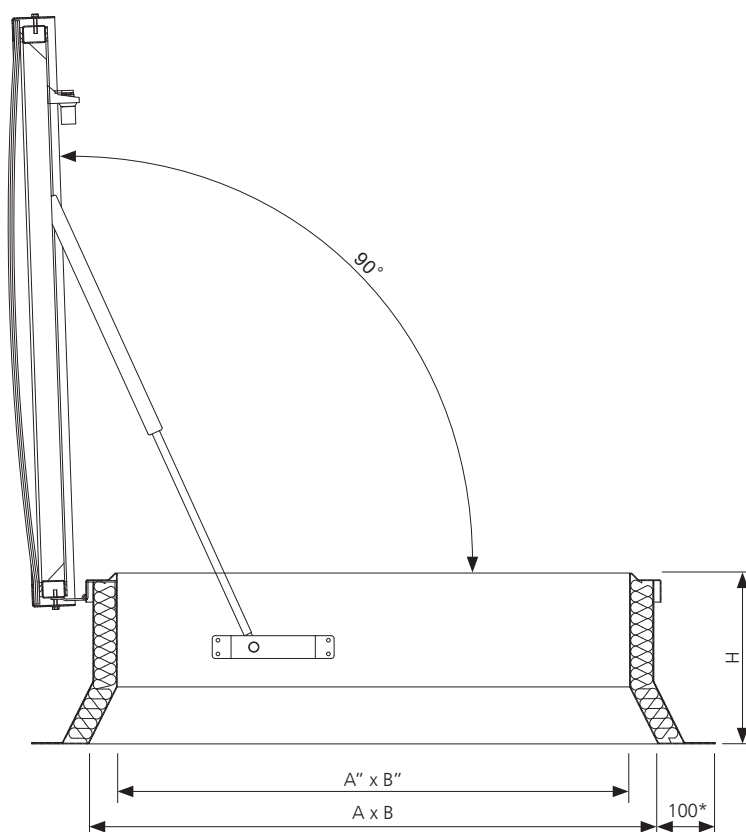
Fig. 26 Section B-B of mcr PROLIGHT NG-A roof hatch in open position, dimensions in mm
