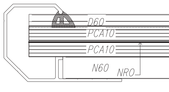
Fig. 133 Section of rooflight of width 1.2÷3.5 m; supporting profile (N) and pressing profile (D) of width 60 mm
