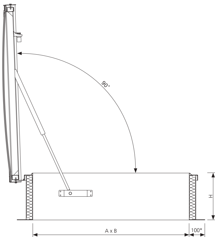
Fig. 23 Section B-B of mcr PROLIGHT C roof hatch in open position, dimensions in mm
