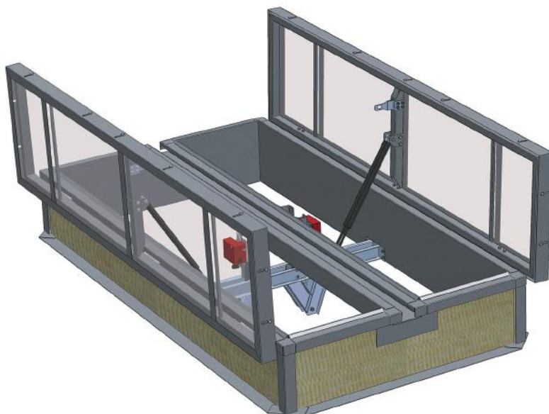
Fig. 79 Design of mcr PROLIGHT DVP smoke vent equipped in mechanic control system
