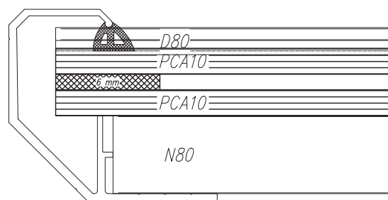
Fig. 118 Section of rooflight of width 3.5÷4.0 m; supporting profile (N) and pressing profile (D) of width 80 mm
