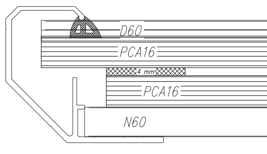
Fig. 122 Section of rooflight of width 1.5÷4.0 m; supporting profile (N) and pressing profile (D) of width 60 mm
