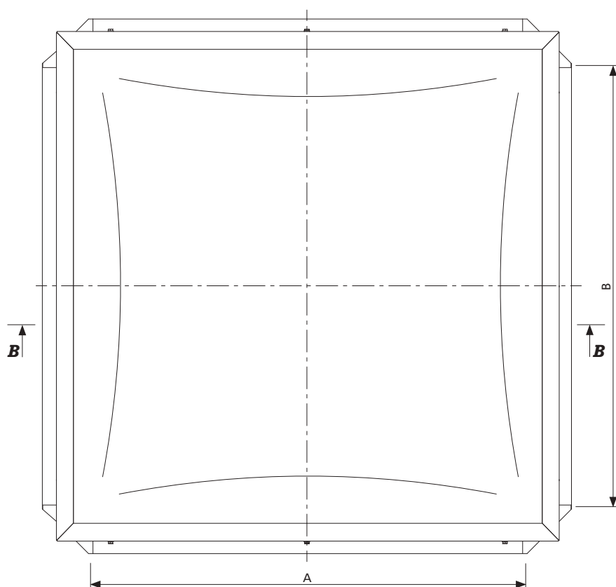
Fig. 18 Top view of mcr PROLIGHT C or E fixed skylight, dimensions in mm
