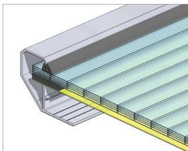
Fig. 125 Rooflight glazing: multi-chamber polycarbonate panel (PCA 10), NRO panel with air gap between (PP)
