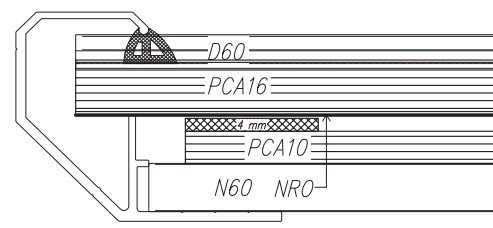
Fig. 138 Section of rooflight of width 1.5÷6.0 m; supporting profile (N) and pressing profile (D) of width 60 mm
