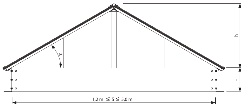
Fig. 100 Cross section A-A of mcr PROLIGHT pyramid skylight
