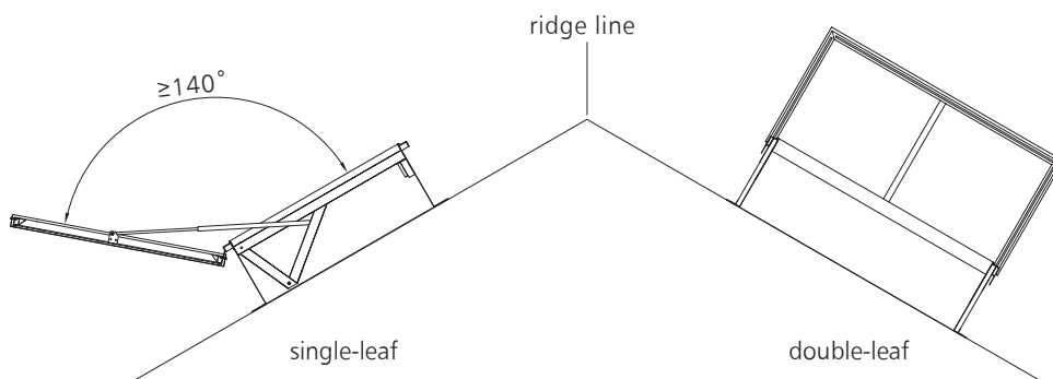
Fig. 34 Side cross-sectional view of the roof
