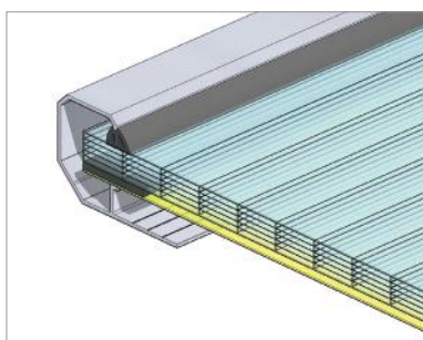
Fig. 128 Rooflight glazing: multi-chamber polycarbonate panel (PCA 16), NRO panel with air gap between (PP)
