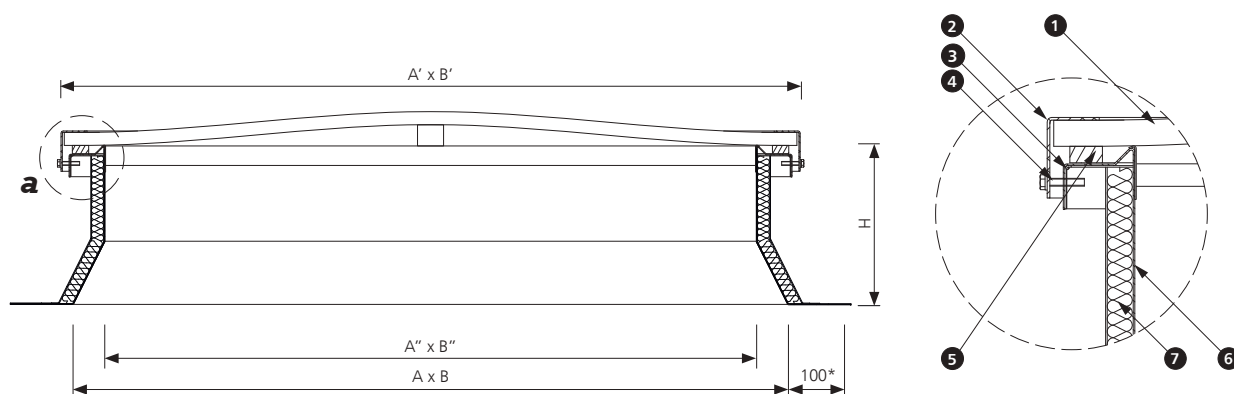
Fig. 20 Section B-B of mcr PROLIGHT NG-A fixed skylight, dimensions in mm
