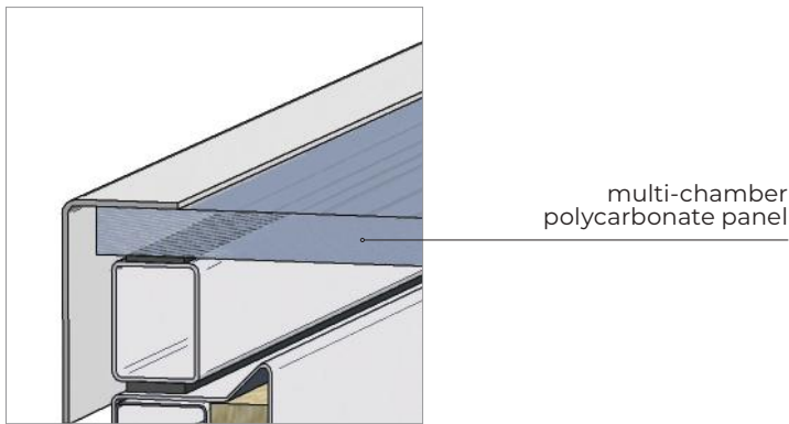
Fig. 36 Vent glazing: multi-chamber polycarbonate panel
