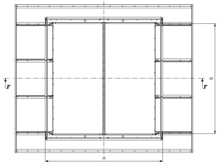
Fig. 91 Top view of arch shaped continuous rooflight with integrated mcr PROLIGHT TB smoke exhaust and daily ventilation single and double-leaf vent
