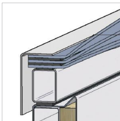
Fig. 45 Vent glazing: triple-layer solid polycarbonate dome
