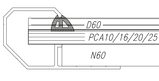
Fig. 108 Rooflight section glazing: single multi-chamber polycarbonate panel
