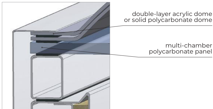
Fig. 53 Vent filling: acrylic dome or solid polycarbonate dome and multi-chamber polycarbonate panel
