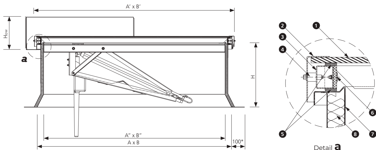
Fig. 5 Section B-B of mcr PROLIGHT NG-A smoke vent in closed position, dimensions in mm
