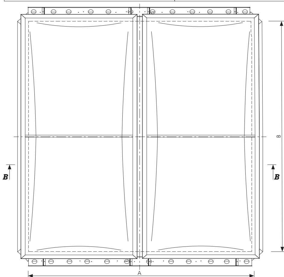
Fig. 12 Top view of mcr PROLIGHT DVP smoke vent in closed position, dimensions in mm
