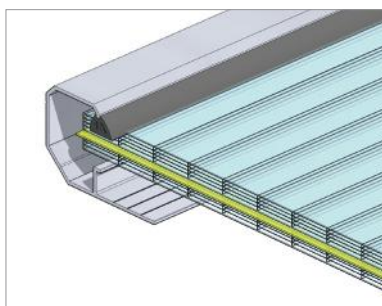
Fig. 132 Rooflight glazing: two multi-chamber polycarbonate panels (PCA 10 + PCA 10) with NRO panel between
