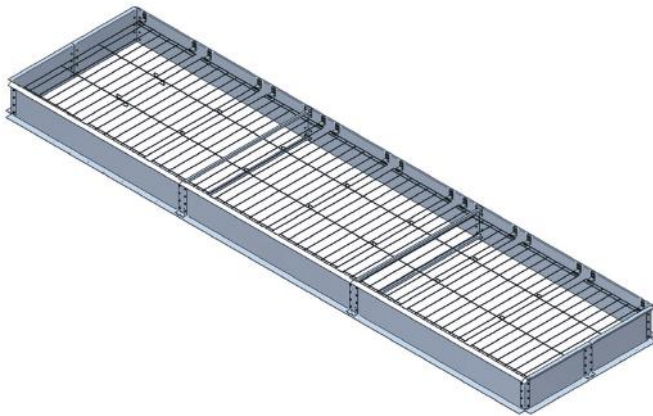
Fig. 142 Safety net 1200 J installed in continuous rooflight base
