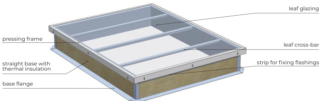
Fig. 16 mcr PROLIGHT E fixed skylight design
