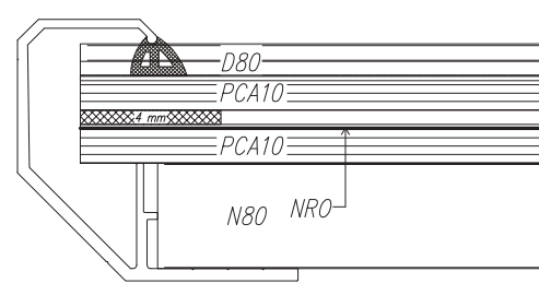
Fig. 136 Section of rooflight of width 4.0 m; multi-chamber polycarbonate panel (PCA), NRO panel
