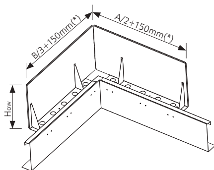
Fig. 65 Internal view of the deflector in the mcr PROLIGHT C/E/NG-A smoke vent
