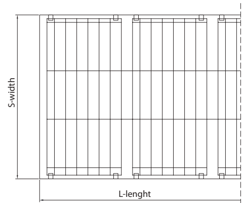
Fig. 143 Top view of safety net installed in continuous rooflight
