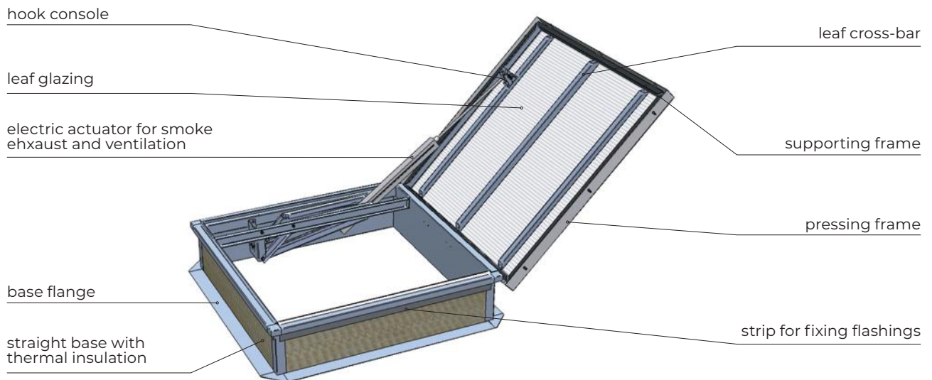
Fig. 57 Design of mcr PROLIGHT smoke vent with an offset electric control system for smoke exhaust and ventilation, featuring a roof access option
