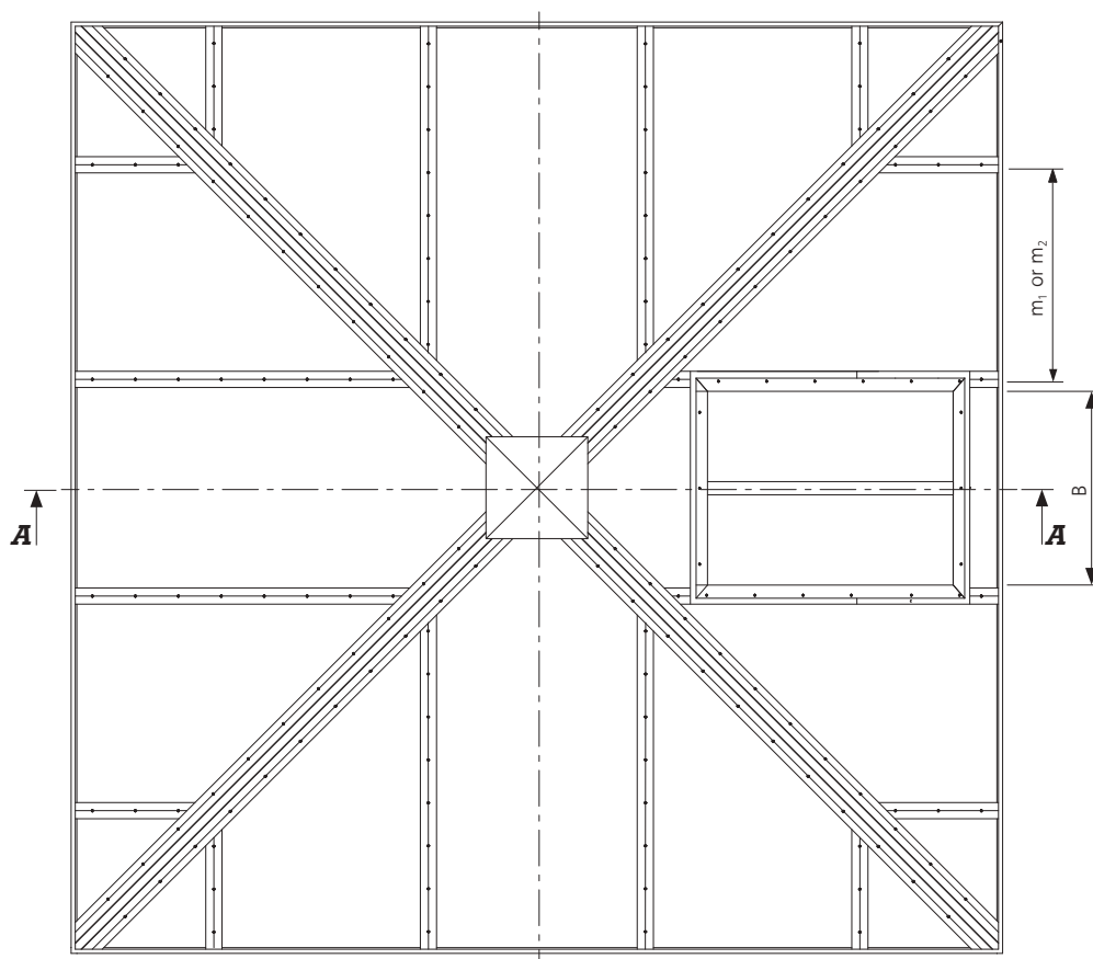
Fig. 103 Top view of mcr PROLIGHT pyramid skylight with daily ventilation vent
