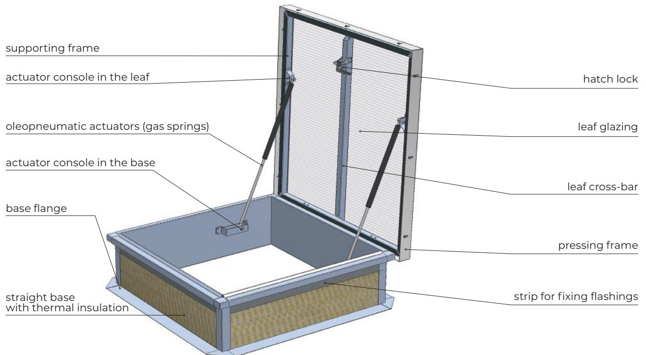
Fig. 22 mcr PROLIGHT C roof hatch design
