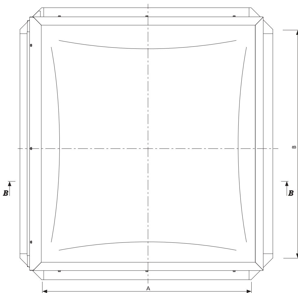
Fig. 30 Top view of mcr PROLIGHT E ventilation vent in open position, dimensions in mm
