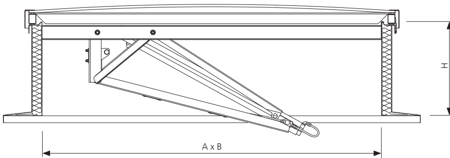
Fig. 75 Section of mcr PROLIGHT E type vent with N plinth type base
