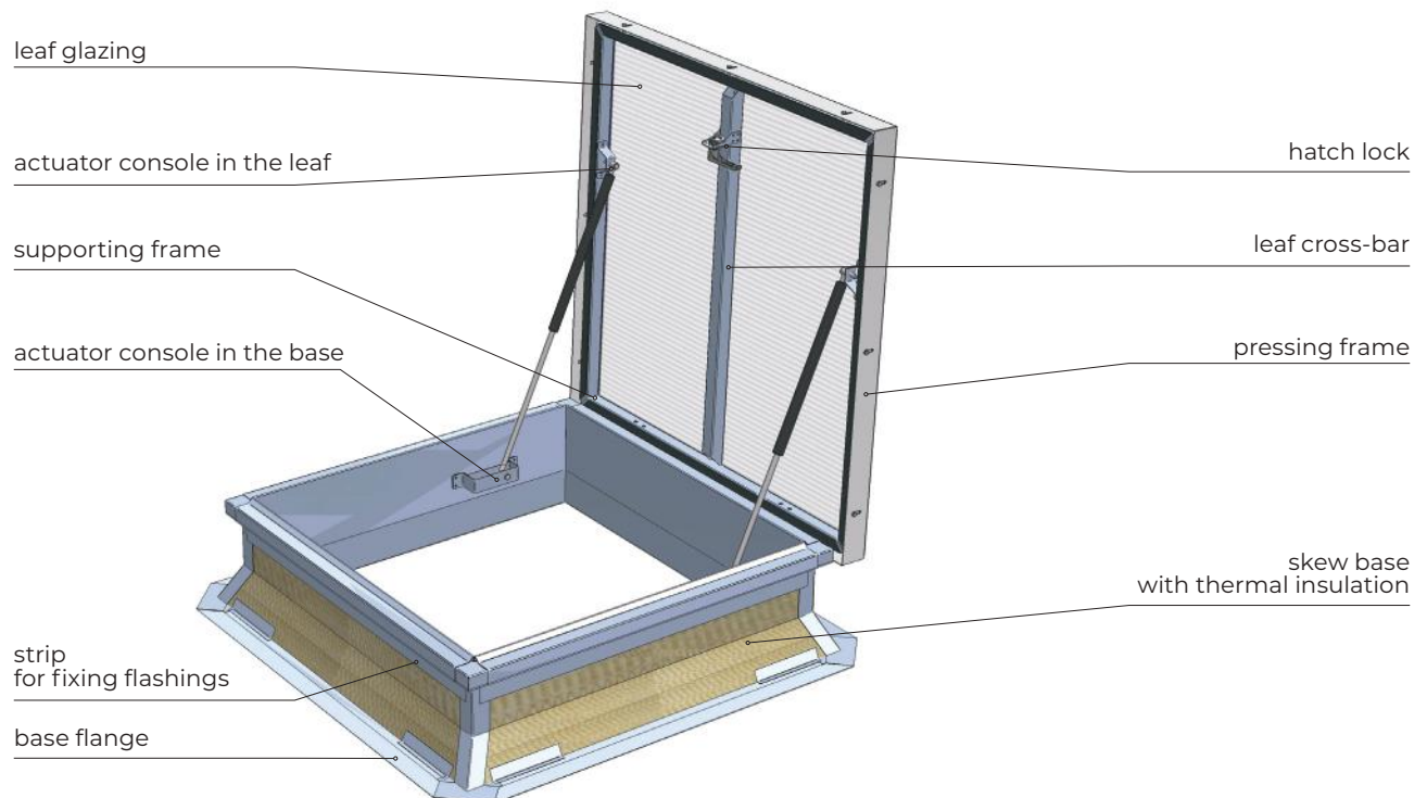
Fig. 25 mcr PROLIGHT NG-A roof hatch design
