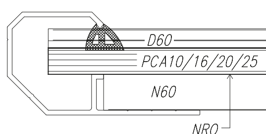
Fig. 124 Rooflight section; glazing – single multi-chamber polycarbonate panel and NRO panel
