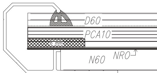
Fig. 126 Section of rooflight of width 1.2÷3.5 m; supporting profile (N) and pressing profile (D) of width 60 mm
