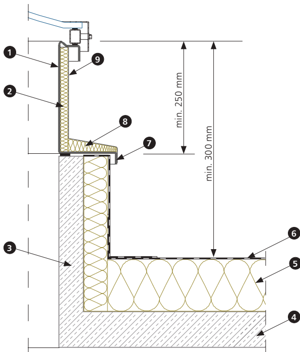
Fig. 75 Section of mcr PROLIGHT E type vent with N plinth type base
