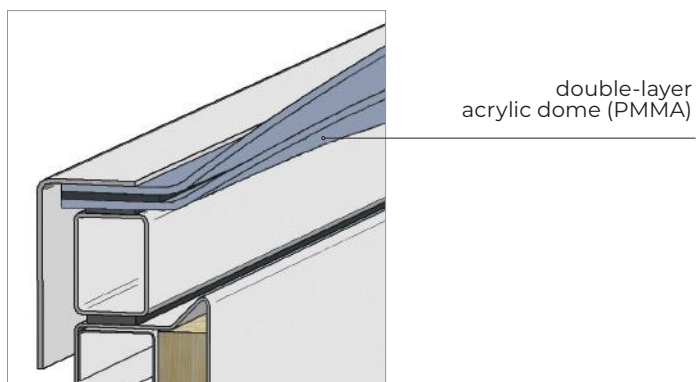
Fig. 39 Vent glazing: double-layer acrylic dome
