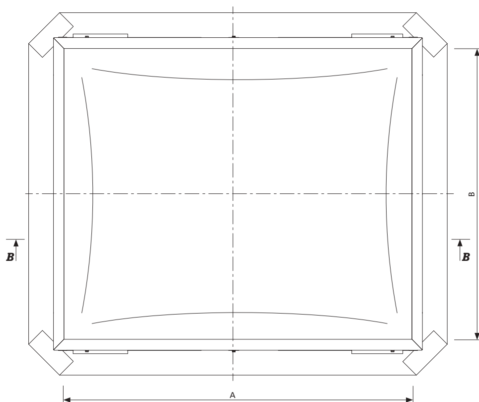
Fig. 21 Top view of mcr PROLIGHT NG-A fixed skylight, dimensions in mm
