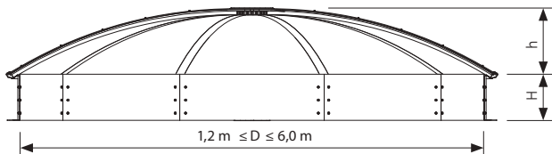
Fig. 105 Cross section A-A of mcr PROLIGHT dome skylight
