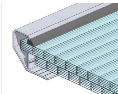
Fig. 114 Rooflight glazing: two multi-chamber polycarbonate panels (PCA 16 + PCA 16)
