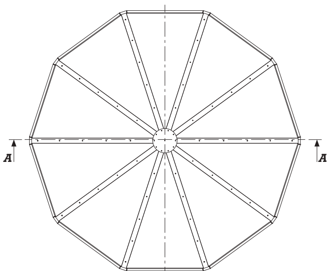
Fig. 106 Top view of mcr PROLIGHT dome skylight
