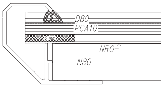
Fig. 127 Section of rooflight of width 1.5÷4.0 m; supporting profile (N) and pressing profile (D) of width 80 mm
