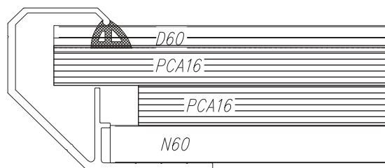
Fig. 115 Section of rooflight of width 1.5÷6.0 m; supporting profile (N) and pressing profile (D) of width 60 mm
