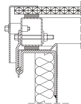
Fig. 38 Vent section, glazing: structured multi-chamber polycarbonate panel
