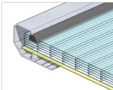
Fig. 123 Rooflight glazing: multi-chamber polycarbonate panel (PCA), NRO panel
