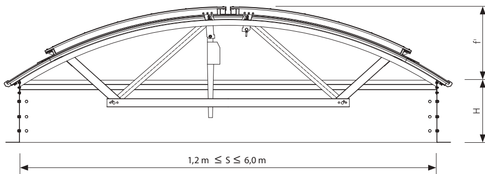
Fig. 85 Cross section C-C of mcr PROLIGHT arch shaped continuous rooflight with integrated smoke exhaust and daily ventilation single-leaf vent
