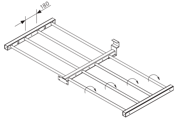
Fig. 71 Anti-burglar grid for smoke vent
