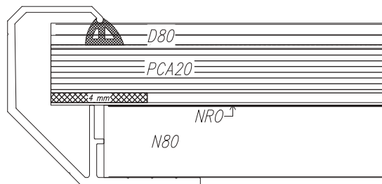
Fig. 131 Section of rooflight of width 2.0÷4.0 m; supporting profile (N) and pressing profile (D) of width 60 mm
