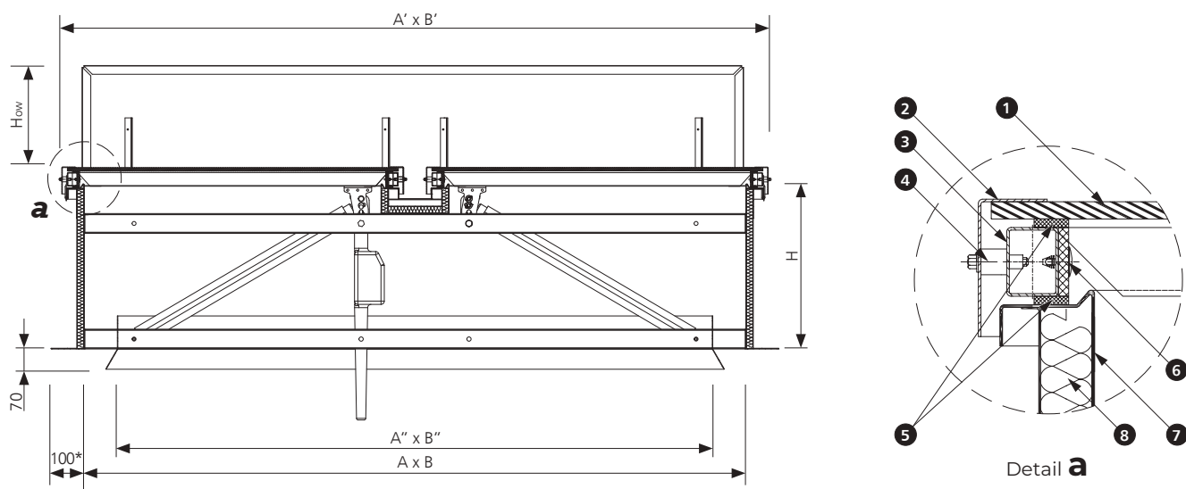
Fig. 11 Section B-B of mcr PROLIGHT DVP smoke vent in closed position, dimensions in mm
