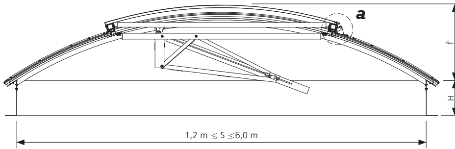
Fig. 89 Cross section E-E of arch shaped continuous rooflight with integrated mcr PROLIGHT TB smoke exhaust and daily ventilation single-leaf vent
