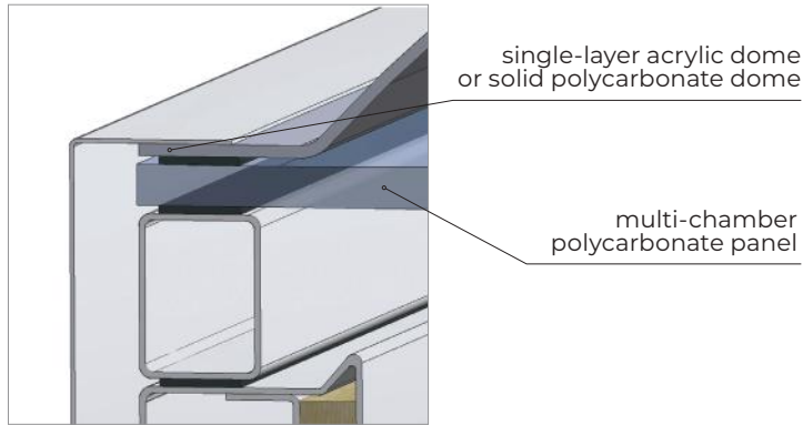
Fig. 51 Vent filling: acrylic dome or solid polycarbonate dome and multi-chamber polycarbonate panel
