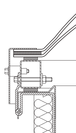
Fig. 40 Vent section, glazing: double-layer acrylic dome
