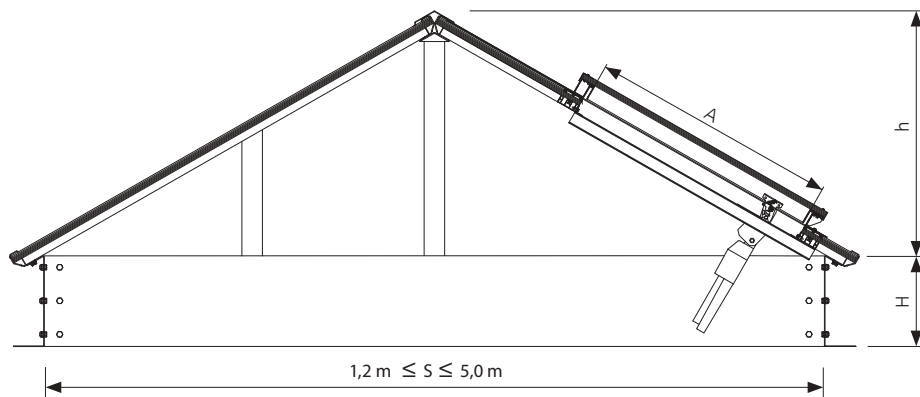
Fig. 102 Cross section A-A of mcr PROLIGHT pyramid skylight with daily ventilation vent
