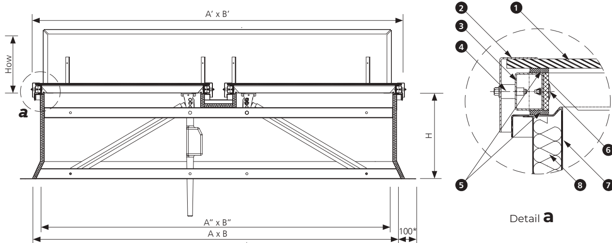
Fig. 14 Section B-B of mcr PROLIGHT DVPS smoke vent in closed position, dimensions in mm
