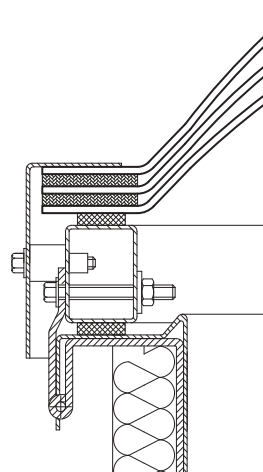
Fig. 46 Vent section, glazing: triple-layer solid polycarbonate dome
