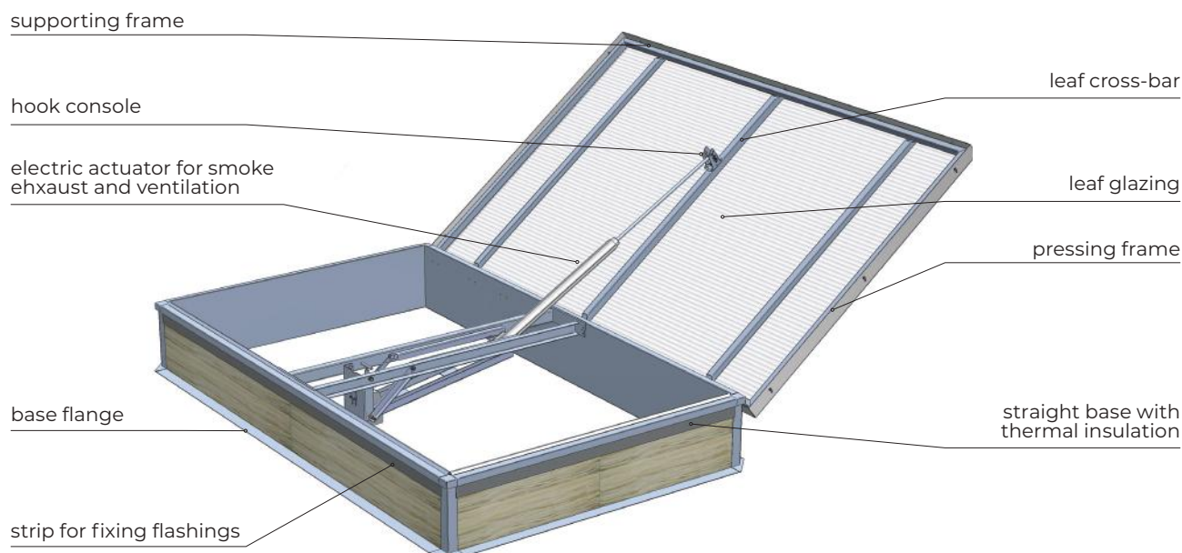
Rys. 60 Design of mcr PROLIGHT E smoke vent with a roof access option, featuring electrical control for smoke exhaust and ventilation, equipped with a single electric actuator mounted symmetrically for side lengths 1800 mm
