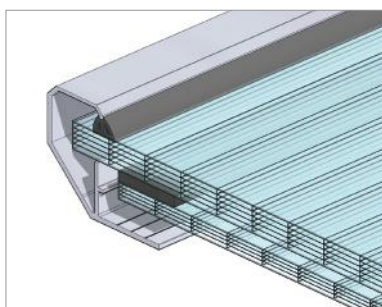
Fig. 119 Rooflight glazing: two multi-chamber polycarbonate panels (PCA 16 + PCA 10) with air gap between (PP)
