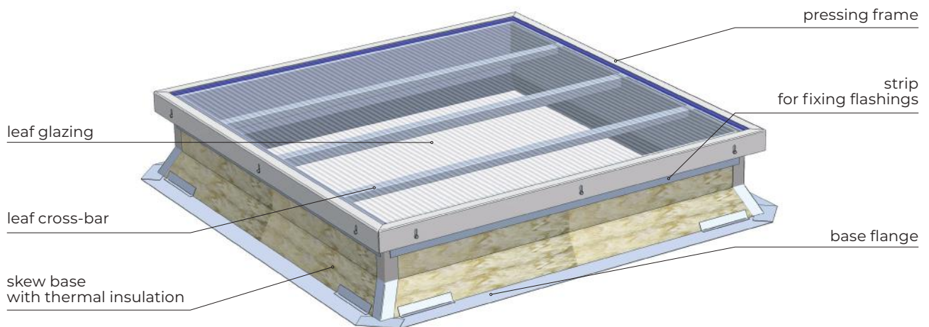
Fig. 19 mcr PROLIGHT NG-A fixed skylight design
