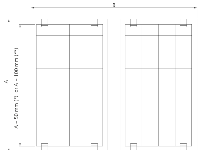
Fig. 73 Top view of vent with safety net
