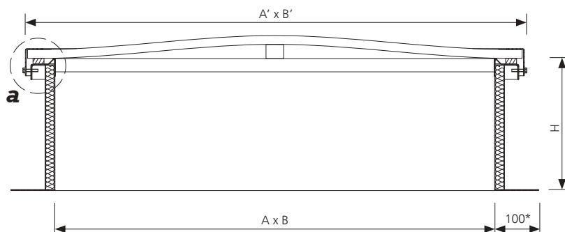
Fig. 17 Section B-B of mcr PROLIGHT C or E fixed skylight, dimensions in mm
