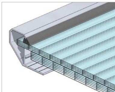
Fig. 112 Rooflight glazing: two multi-chamber polycarbonate panels (PCA 10 + PCA 16)
