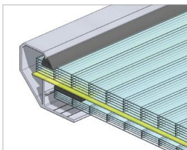
Fig. 137 Rooflight glazing: two multi-chamber polycarbonate panels (PCA 16 + PCA 10) with NRO panel and air gap (PP) between
