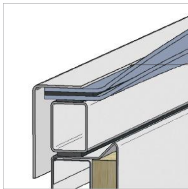
Fig. 43 Vent glazing: double-layer solid polycarbonate dome
