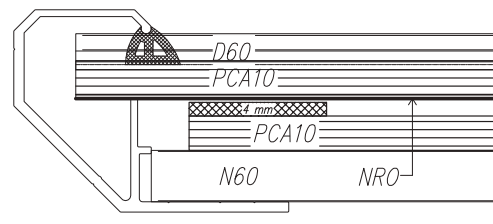
Fig. 135 Section of rooflight of width 1.2÷3.5 m; supporting profile (N) and pressing profile (D) of width 60 mm
