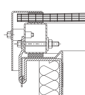
Fig. 56 Vent section, glazing: B ROOF (t1)
