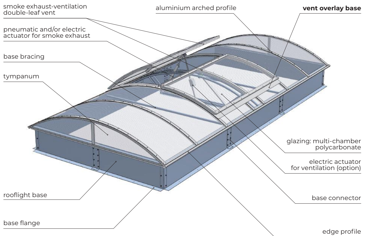
Fig. 84 Design of mcr PROLIGHT arch shaped continuous rooflight with integrated smoke exhaust and daily ventilation double-leaf vent
