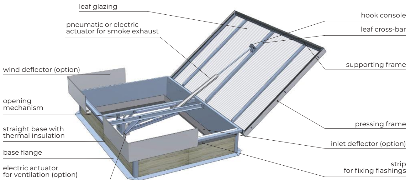
Fig. 1 Design of mcr PROLIGHT E smoke vent equipped with wind deflectors and inlet deflector, with pneumatic actuator for smoke exhaust and electric actuator for ventilation
