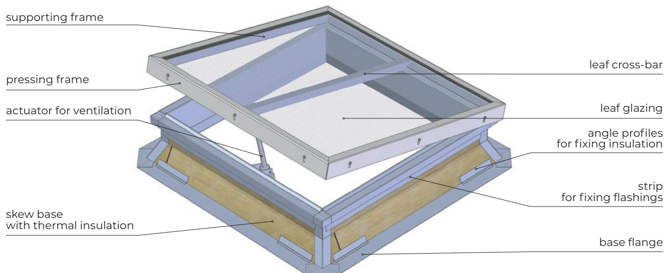
Fig. 31 mcr PROLIGHT C ventilation vent design with electric actuator for ventilation
