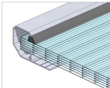
Fig. 107 Rooflight glazing: multi-chamber polycarbonate panel (PCA)
