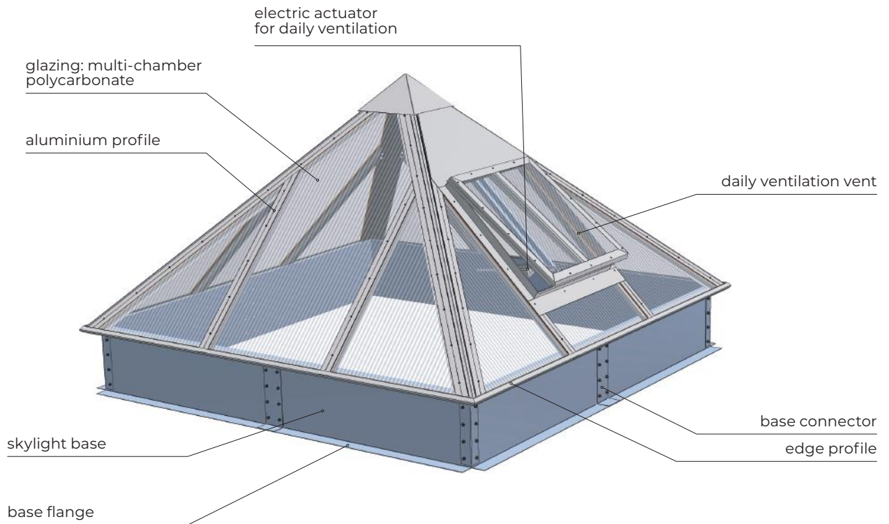
Fig. 99 Design of mcr PROLIGHT pyramid skylight with smoke vent, with electric actuator for daily ventilation
