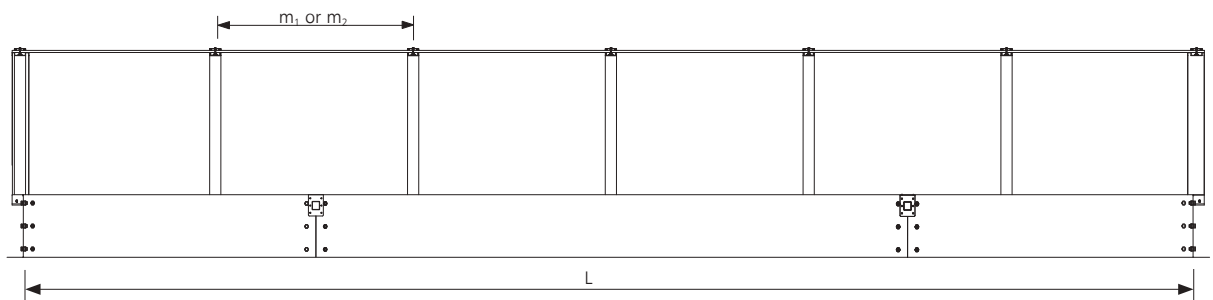
Fig. 94 Cross section B-B of mcr PROLIGHT triangular shaped continuous rooflight
