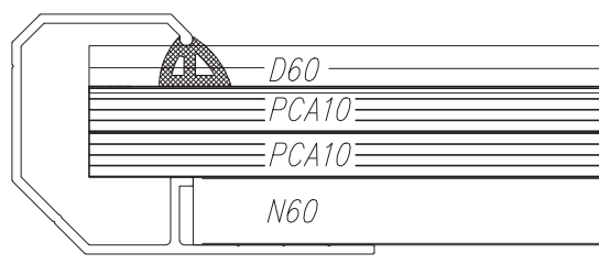
Fig. 110 Section of rooflight of width 1.2 ÷ 3.5 m; supporting profile (N) and pressing profile (D) of width 60 mm
