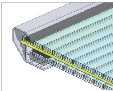
Fig. 134 Rooflight glazing: two multi-chamber polycarbonate panels (PCA 10 + PCA 10) with air gap (PP) and NRO panel between
