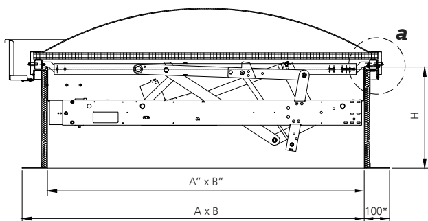
Rys. 7 Cross-section B-B through the mcr PROLIGHT C smoke vent in the closed position, dimensions in mm
