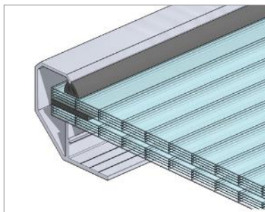
Fig. 116 Rooflight glazing: two multi-chamber polycarbonate panels (PCA 10 + PCA 10) with air gap between (PP)
