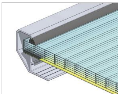
Fig. 130 Rooflight glazing: multi-chamber polycarbonate panel (PCA 10), NRO panel with air gap between (PP)
