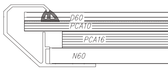
Fig. 113 Section of rooflight of width 1.5÷4.0 m; supporting profile (N) and pressing profile (D) of width 60 mm
