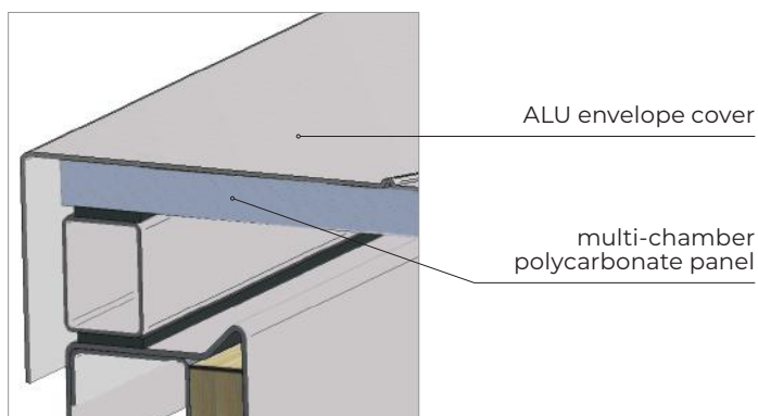
Fig. 49 Vent glazing: ALU envelope cover with multi-chamber polycarbonate
