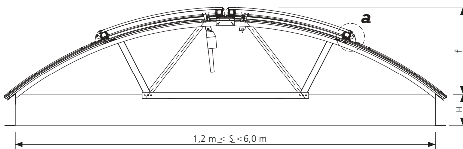
Fig. 90 Cross section F-F of arch shaped continuous rooflight with integrated mcr PROLIGHT TB smoke exhaust and daily ventilation double-leaf vent
