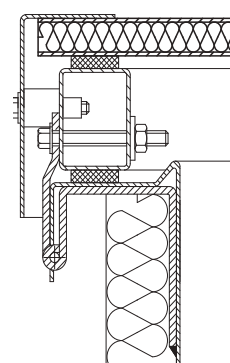
Fig. 48 Vent section, glazing: ALU sandwich panel
