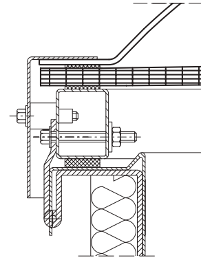
Fig. 52 Vent section, glazing: acrylic dome or solid polycarbonate dome and multi-chamber polycarbonate panel
