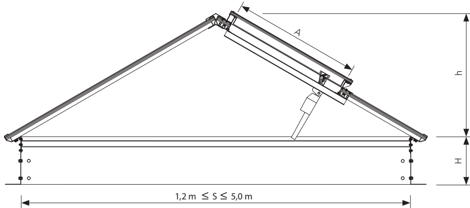
Fig. 96 Cross section C-C of mcr PROLIGHT triangular shaped continuous rooflight with daily ventilation single-leaf vent
