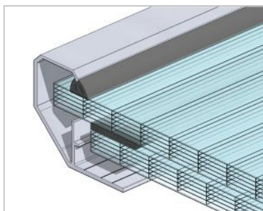
Fig. 121 Rooflight glazing: two multi-chamber polycarbonate panels (PCA 16 + PCA 16) with air gap between (PP)
