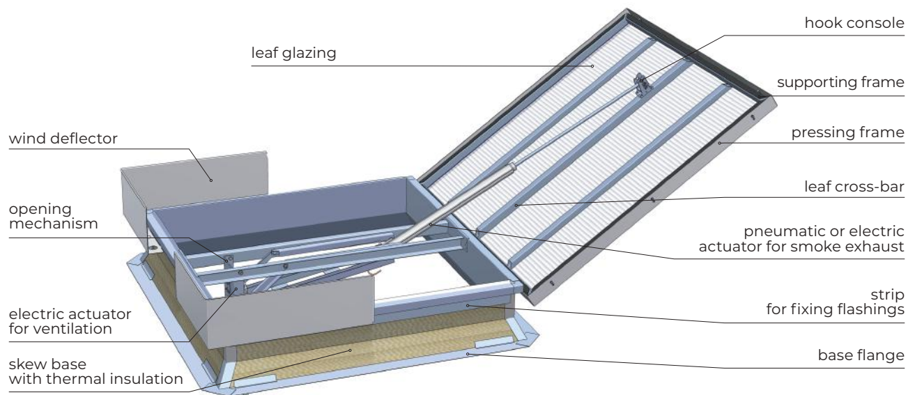
Fig. 4 Design of mcr PROLIGHT NG-A smoke vent equipped with wind deflectors, with pneumatic actuator for smoke exhaust and electric actuator for ventilation
