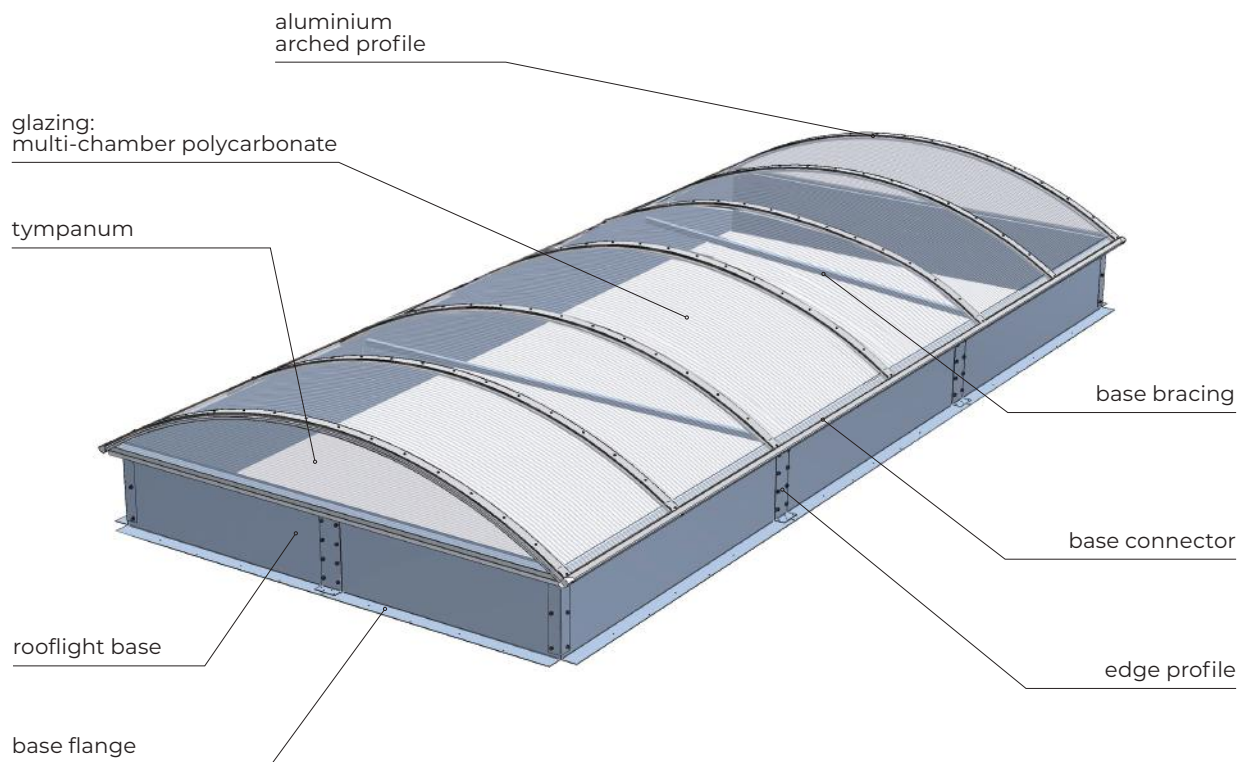
Fig. 80 Design of mcr PROLIGHT arch shaped continuous rooflight
