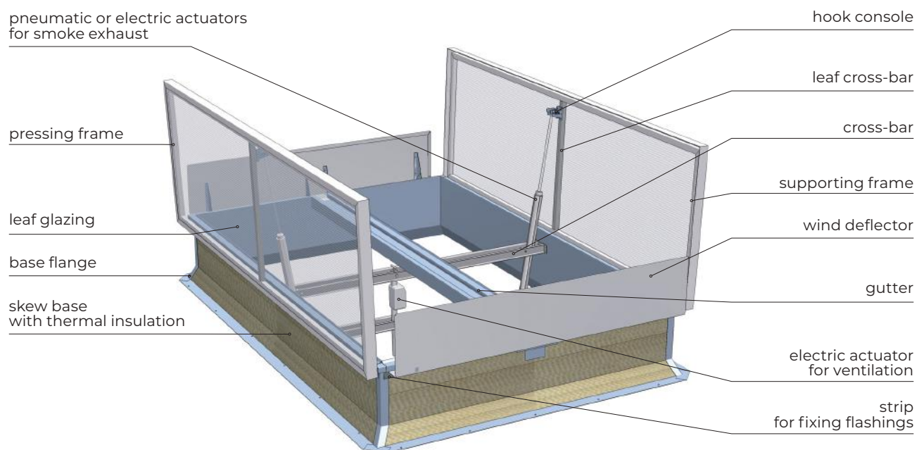
Fig. 13 Design of mcr PROLIGHT DVPS smoke vent equipped with wind deflectors, with pneumatic actuators for smoke exhaust and electric actuator for ventilation
