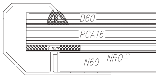
Fig. 129 Section of rooflight of width 1.5÷4.0 m; supporting profile (N) and pressing profile (D) of width 60 mm
