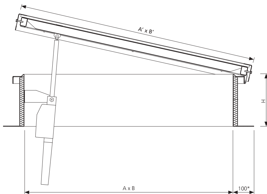
Fig. 29 Section B-B of mcr PROLIGHT E ventilation vent in open position, dimensions in mm
