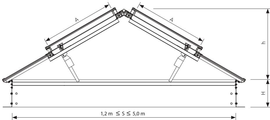
Fig. 97 Cross section D-D of mcr PROLIGHT triangular shaped continuous rooflight with daily ventilation double-leaf vent
