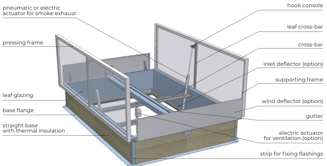
Fig. 10 Design of mcr PROLIGHT DVP smoke vent equipped with wind deflectors and inlet deflector, with pneumatic actuators for smoke exhaust and electric actuator for ventilation.
