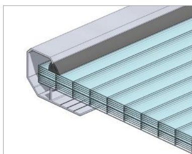
Fig. 109 Rooflight glazing: two multi-chamber polycarbonate panels (PCA 10 + PCA 10)
