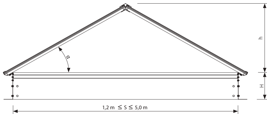
Fig. 93 Cross section A-A of mcr PROLIGHT triangular shaped continuous rooflight
