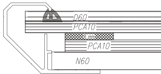
Fig. 117 Section of rooflight of width 1.2÷3.5 m; supporting profile (N) and pressing profile (D) of width 60 mm
