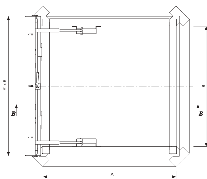
Fig. 27 Top view of mcr PROLIGHT NG-A roof hatch in open position, dimensions in mm
