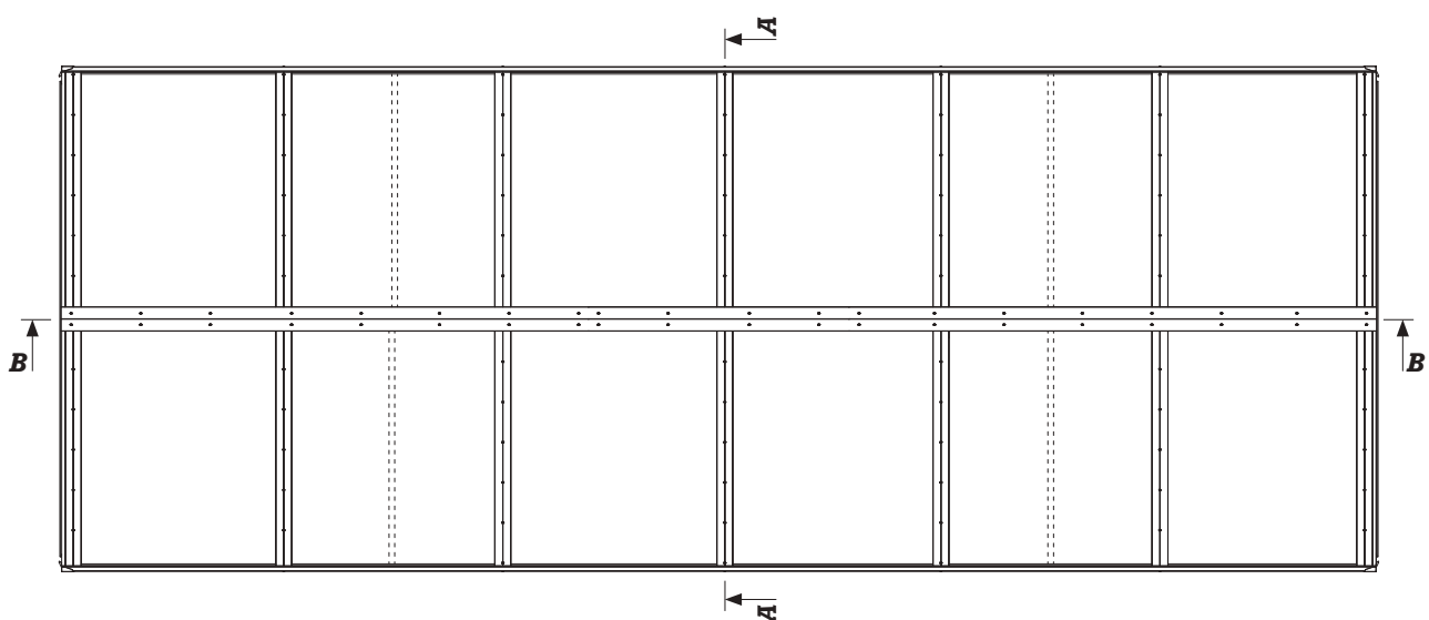
Fig. 95 Top view of mcr PROLIGHT triangular shaped continuous rooflight
