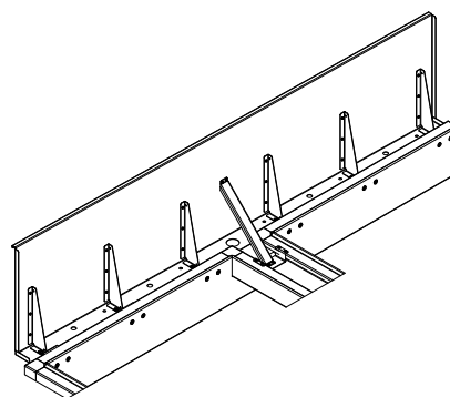
Fig. 66 Internal view of the deflector in the mcr PROLIGHT DVP/DVPS smoke vent
