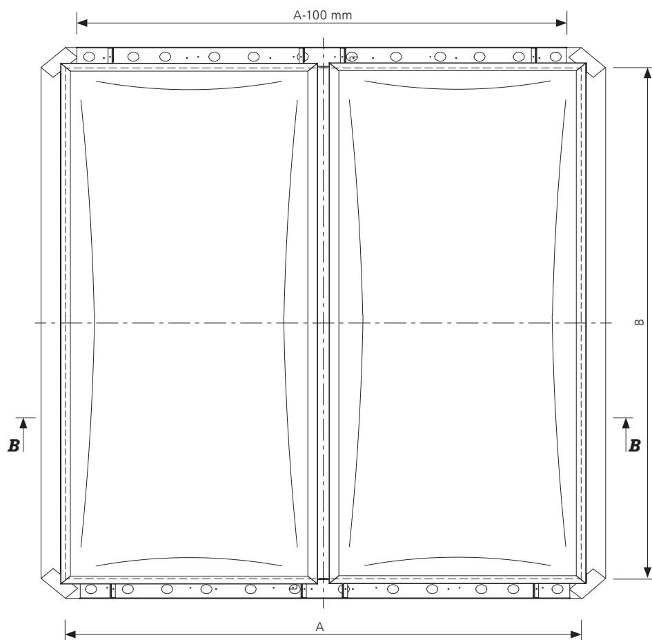
Fig. 15 Top view of mcr PROLIGHT DVPS smoke vent in closed position, dimensions in mm
