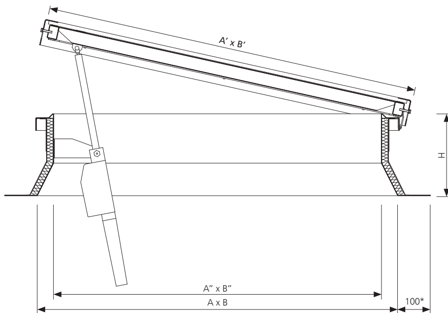
Fig. 32 Section B-B of mcr PROLIGHT NG-A ventilation vent with skew base in open position, dimensions in mm
