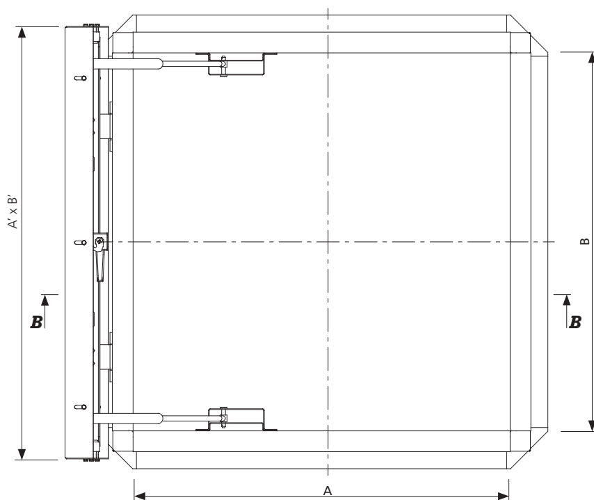
Fig. 24 Top view of mcr PROLIGHT C roof hatch in open position, dimensions in mm
