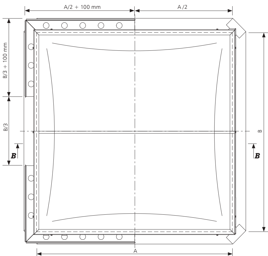
Fig. 6 Top view of mcr PROLIGHT NG-A smoke vent in closed position, dimensions in mm
