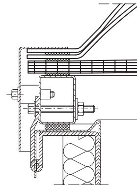
Fig. 54 Vent section, glazing: acrylic dome or solid polycarbonate dome and multi-chamber polycarbonate panel
