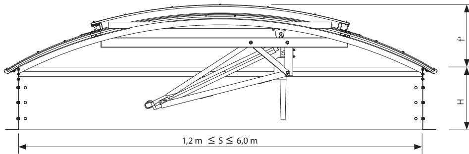
Fig. 85 Cross section C-C of mcr PROLIGHT arch shaped continuous rooflight with integrated smoke exhaust and daily ventilation single-leaf vent
