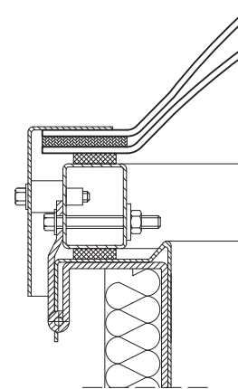
Fig. 44 Vent section, glazing: double-layer solid polycarbonate dome
