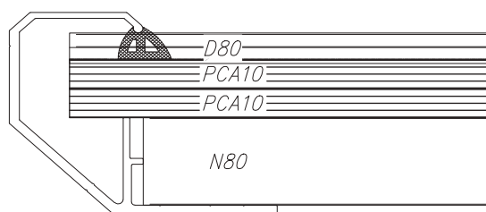
Fig. 111 Section of rooflight of width 3.5 ÷ 4.0 m; supporting profile (N) and pressing profile (D) of width 80 mm
