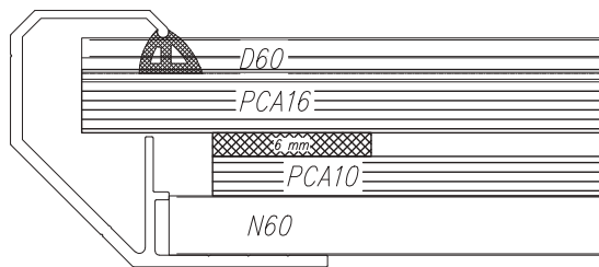
Fig. 120 Section of rooflight of width 1.5÷6.0 m; supporting profile (N) and pressing profile (D) of width 60 mm
