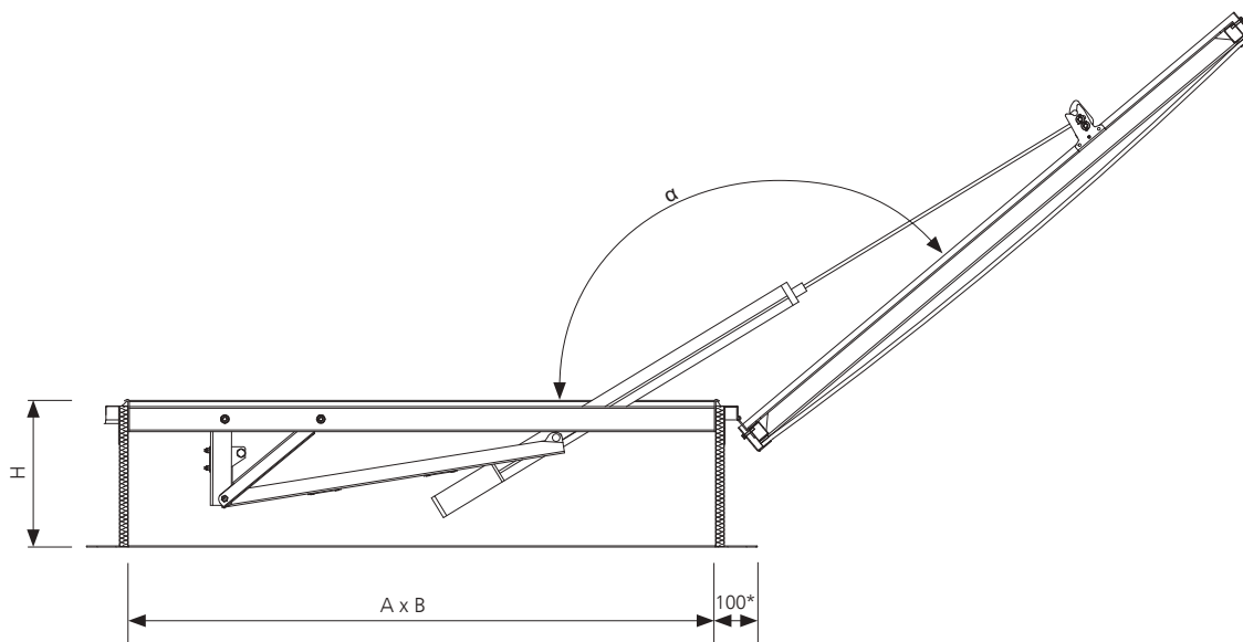
Fig. 58 Section B-B of mcr PROLIGHT smoke vent with roof access function in open position, dimensions in mm
